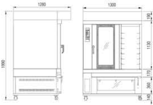
5 trays convection oven+ 1 deck 4 trays deck oven
