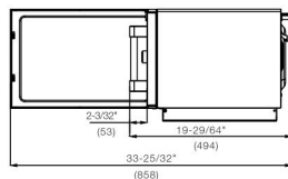
SIDE VIEW (DOOR OPEN)
