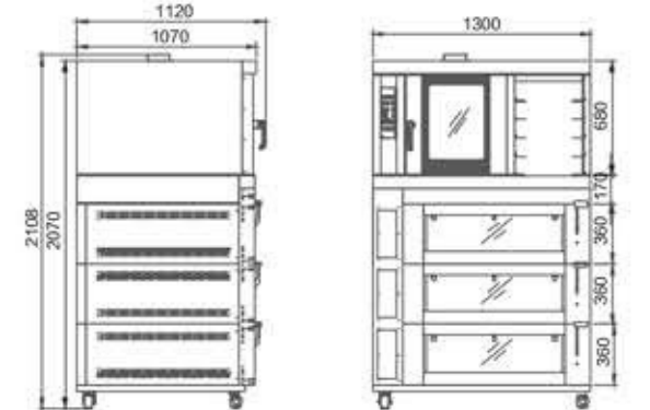
电5盘热风炉+3层6盘电烘炉带层架 5 trays Electric Convection Oven combines with 3 decks 6trays Electric Oven with shelf
