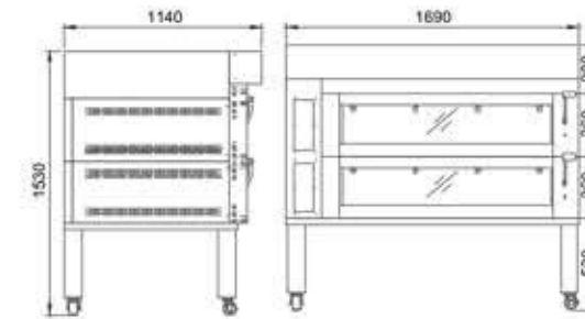
电10盘热风炉+1层2盘电烘炉带层架 10 trays Electric Convection Oven combines with 1 deck 2 trays Electric Oven with shelf
