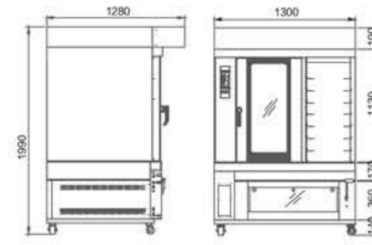
电10盘热风炉+1层2盘电烘炉带层架 10 trays Electric Convection Oven combines with 1 deck 2 trays Electric Oven with shelf
