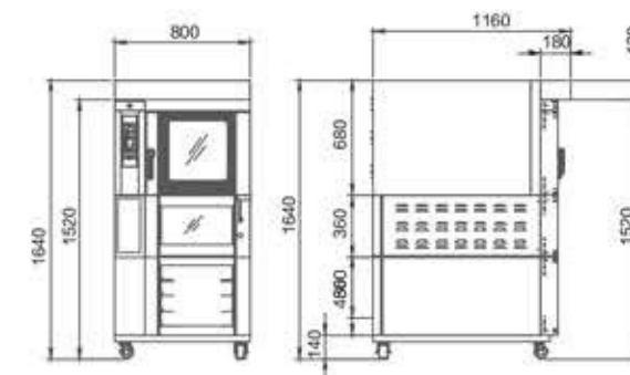
电5盘热风炉+1层1盘电烘炉带层架 5 trays Electric Convection Oven combines with 1 deck 1 tray Electric Oven with shelf
