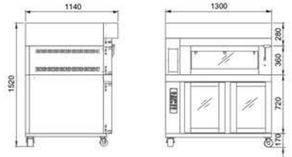
一层二盘电炉带12盘发酵箱 1 deck 2 trays Electric oven with 12 trays proofer
