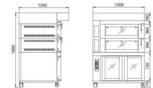
2层4盘带12盘发酵箱 2 decks 4 trays Electric Oven with 12 trays Electric Proofer
