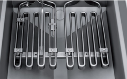
热效率极高且易清洁维护的带状加热管 能够快速回温，实现食物表面金黄酥脆且保持内部水分不流失的效果 Flat-bar heating element transfers heat more efficiently. With snap-action probe, heating element(s) heats up rapidly when it detects a change in the load and/or a drop in temperature, which helps to return to proper temperature faster To achieve the effect that the surface of the food is golden and crispy and keep the internal moisture not lost
