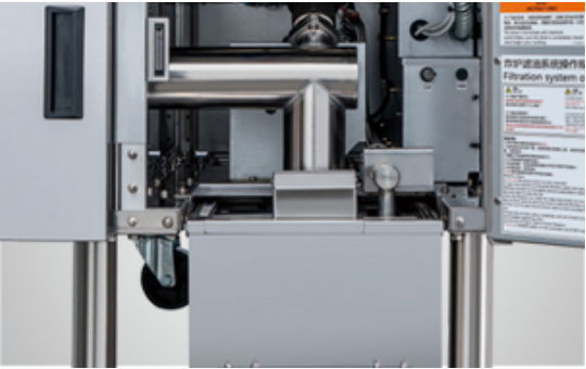
内置滤油系统 不但节约了使用空间，而且在保证烹炸食物保持高质量出品同时，还极大延长了油品的使用寿命，降低运营成本 The built-in oil filtering system not only saves the space, but also ensures that the fried food maintains high-quality outcome, while also greatly extending the service life of the oil and reducing operating costs
