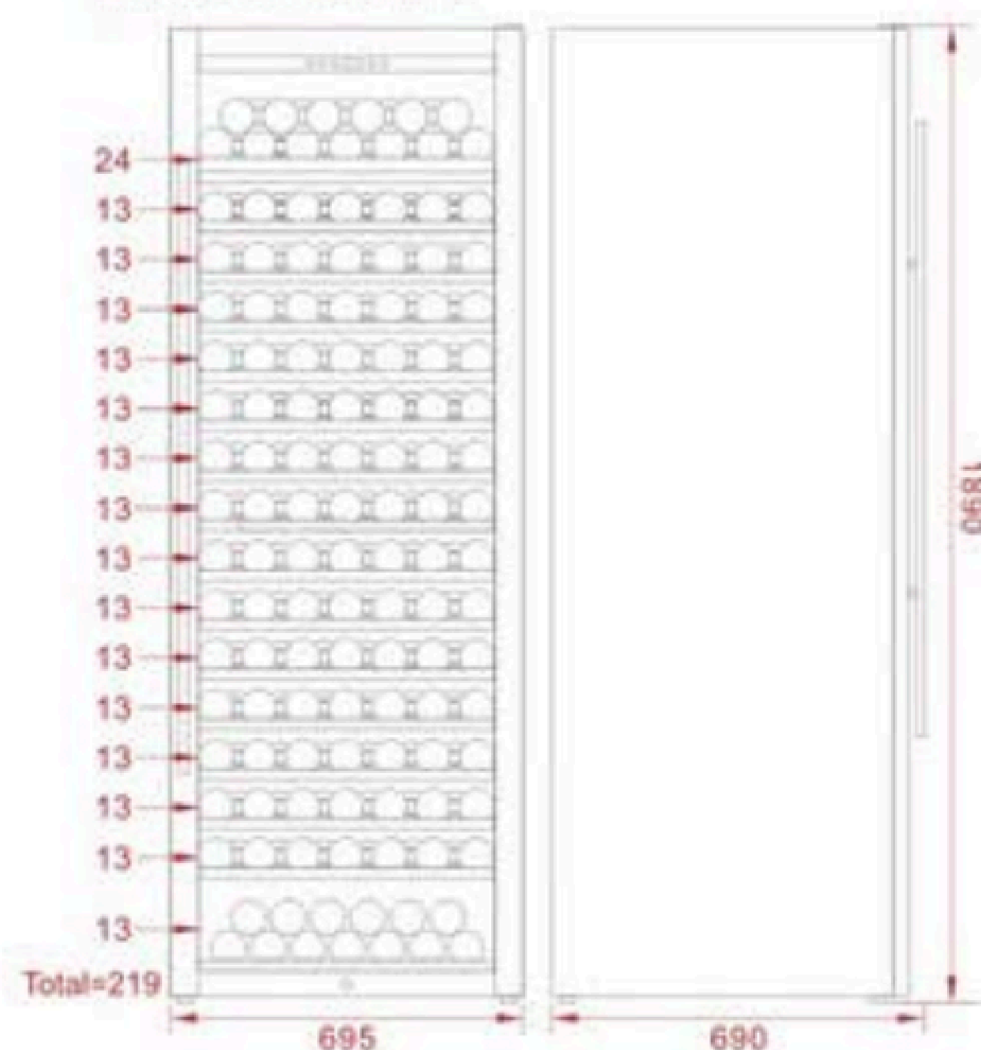
SRW-230S Product(W*D*H)mm
