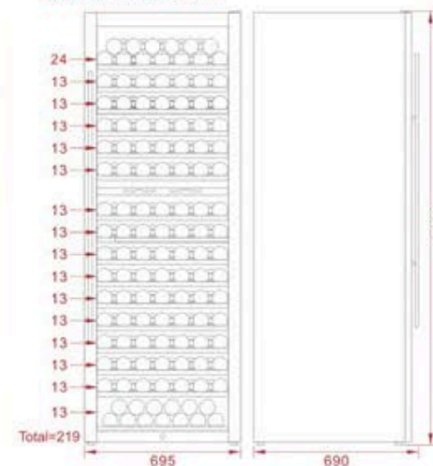
SRW-230D Product(W*D*H)mm
