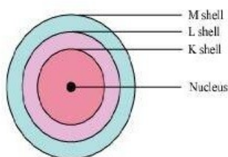
Bohr's model of an atom with three shells
