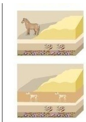
Layers of fossils
