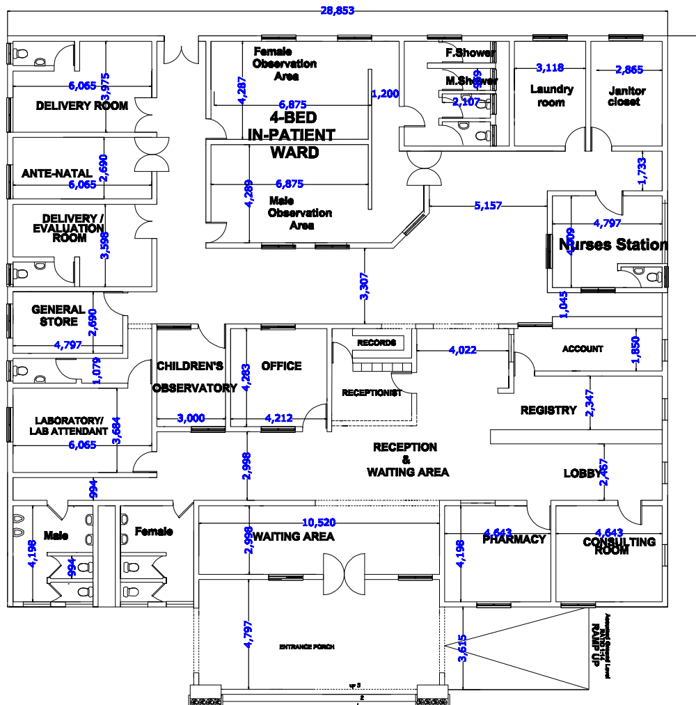
GROUND FLOOR PLAN CLINIC
