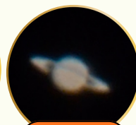
THE PLANETS
