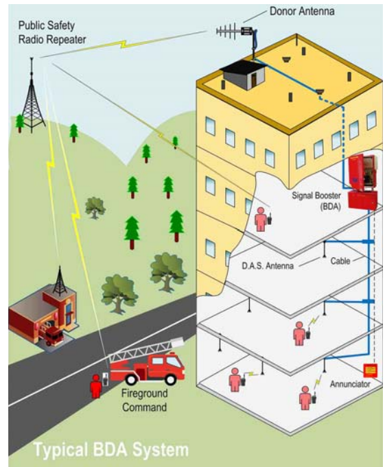
BDA System with Fireground Communication
