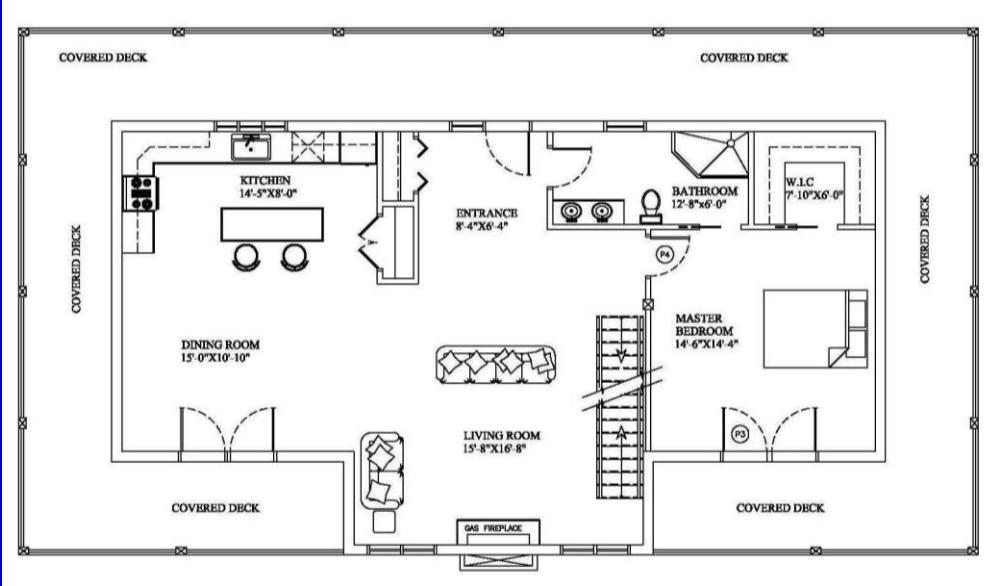
Main floor plan 1144 Sq.Ft
