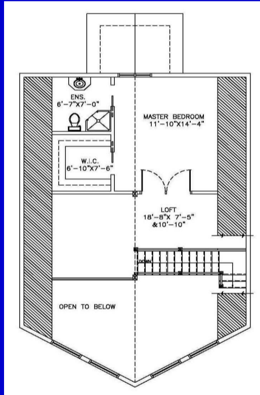
Second floor plan 515 Sq.Ft
