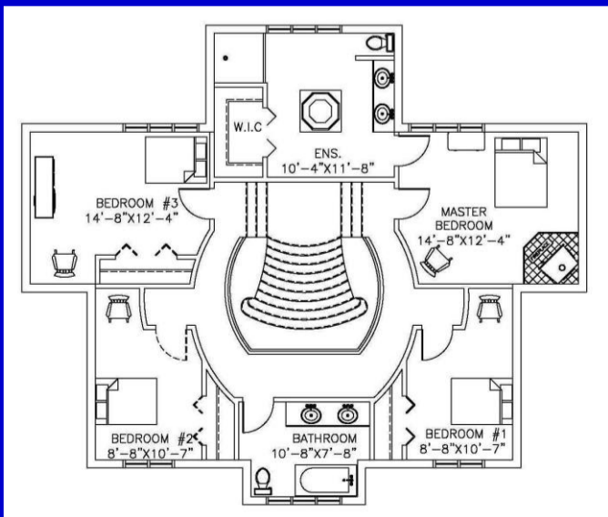
Second floor plan 1180 Sq.Ft
