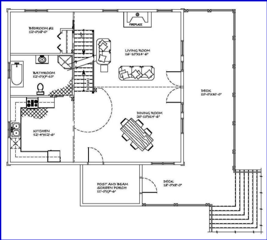
Main floor plan 957 Sq.Ft
