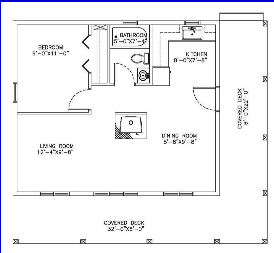
Main floor plan 525 Sq.Ft
