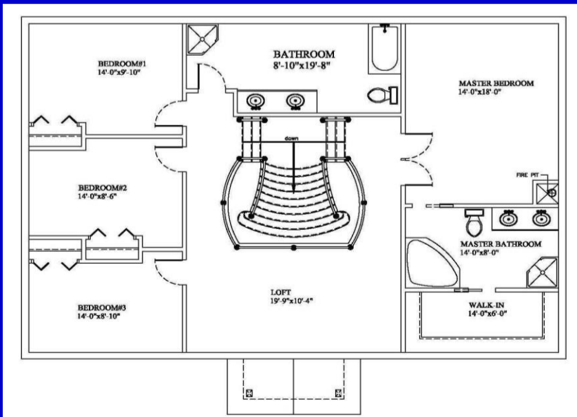
Second floor plan 1250 Sq.Ft
