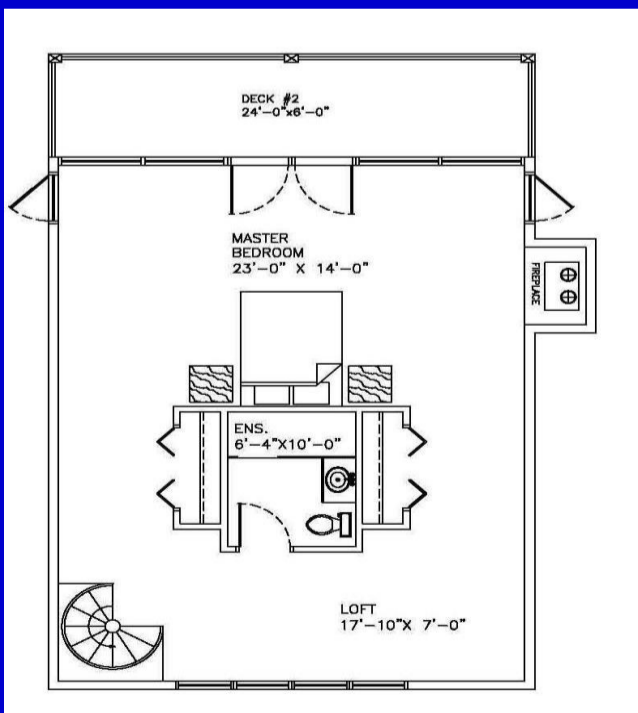
Second floor plan 690 Sq.Ft
