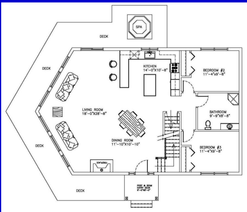
Main floor plan 1235 Sq.Ft
