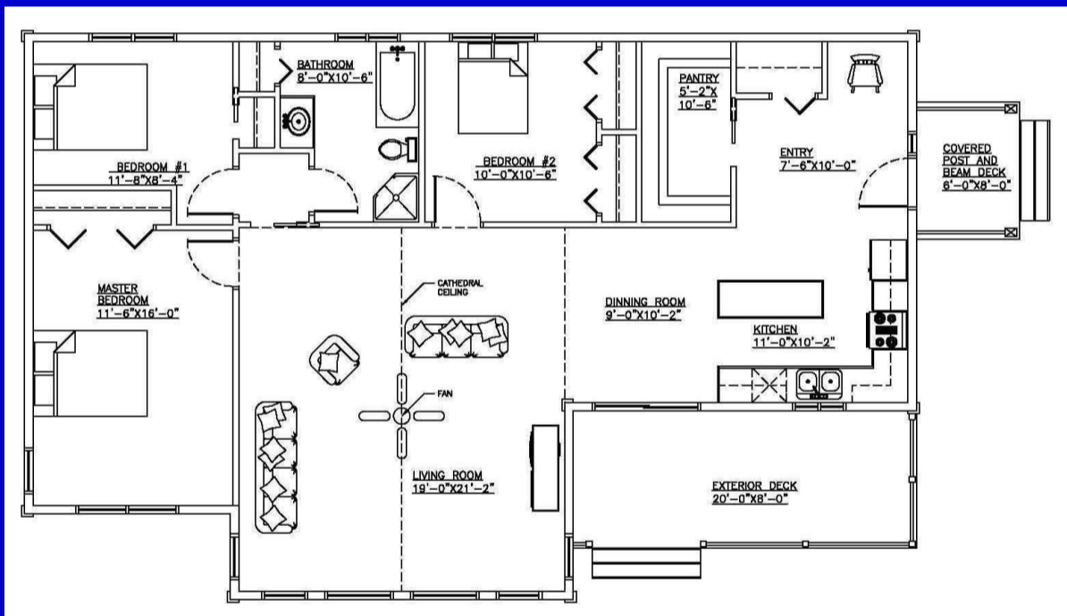
Main floor plan 1352 Sq.Ft
