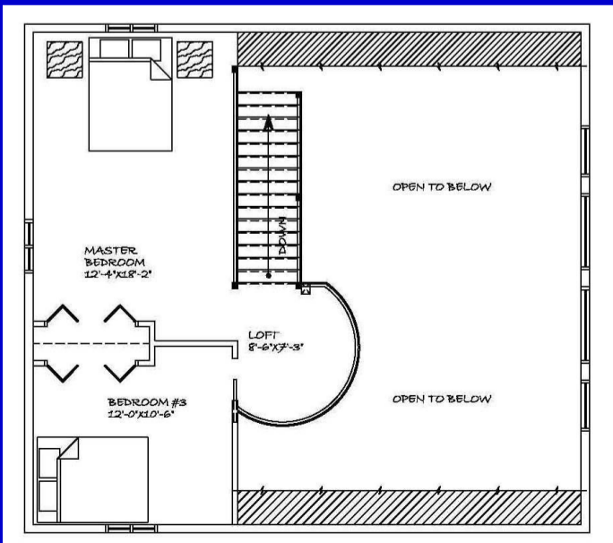
Second floor plan 404 Sq.Ft
