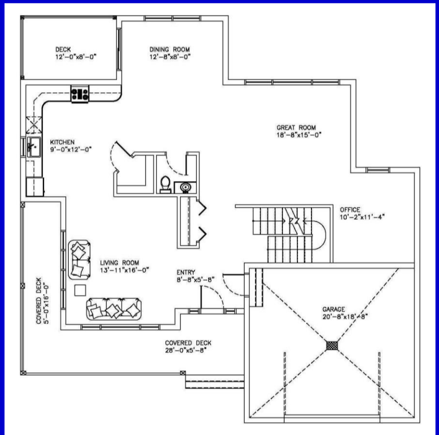
Main floor plan 1211 Sq.Ft
