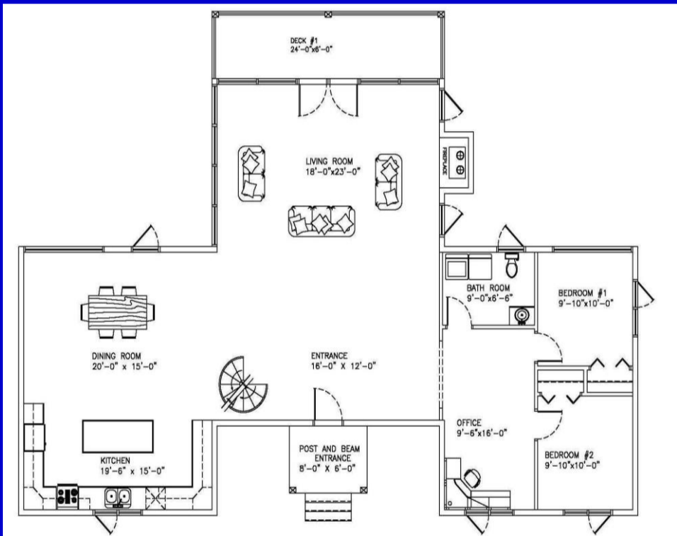
Main floor plan 1602 Sq.Ft
