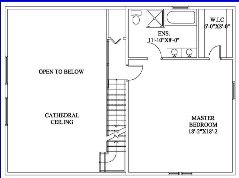
Second floor plan 574 Sq.Ft
