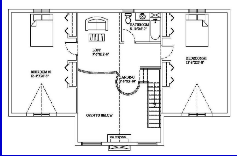
Second floor plan 934 Sq.Ft
