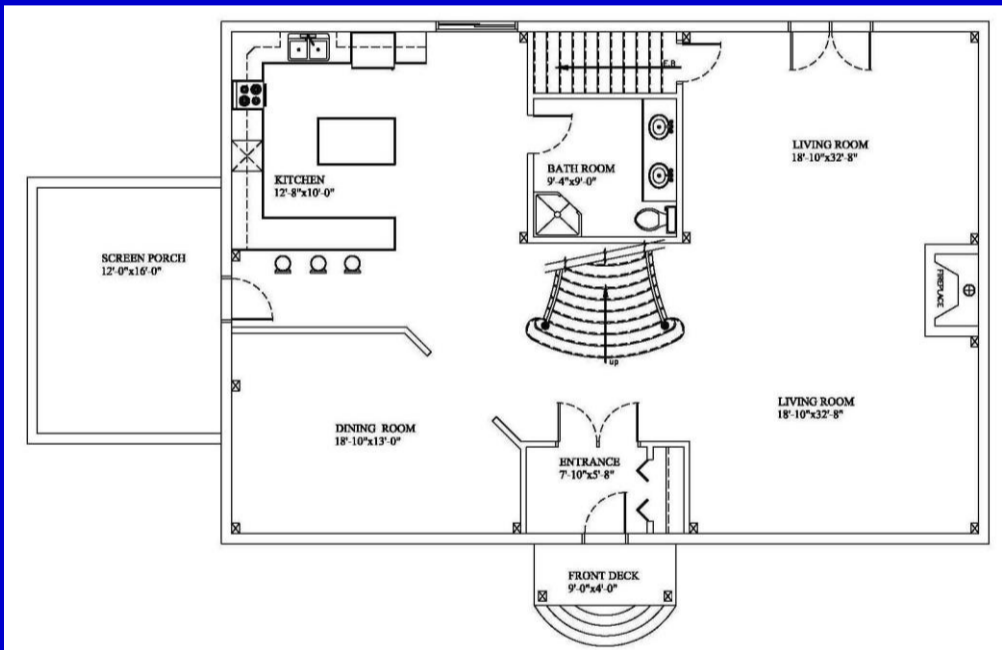
Main floor plan 1395 Sq.Ft
