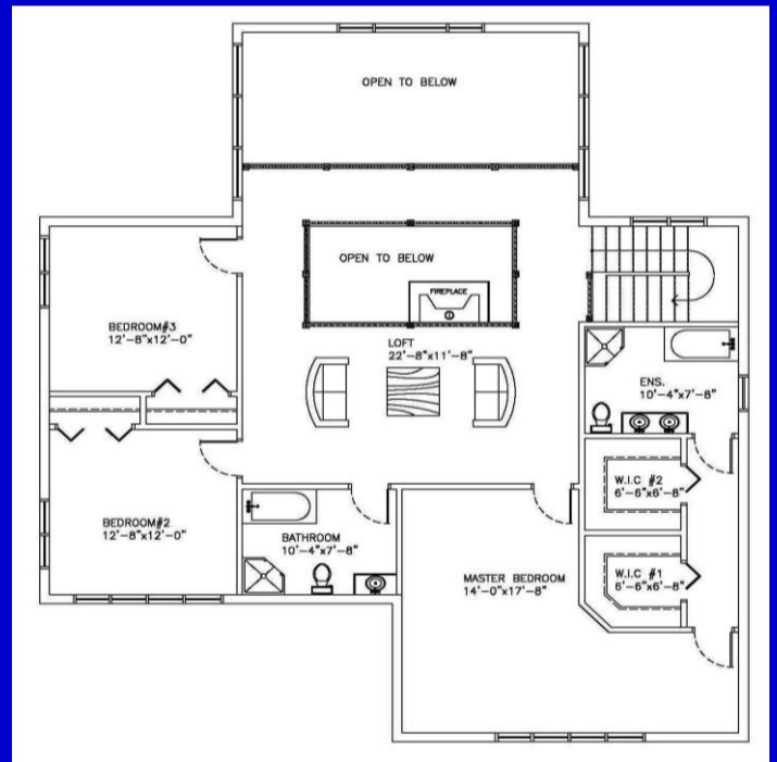
Second floor plan 1469 Sq.Ft
