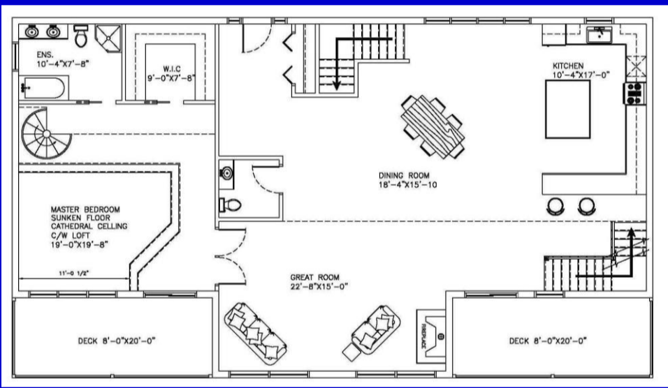
Main floor plan 1852 Sq.Ft
