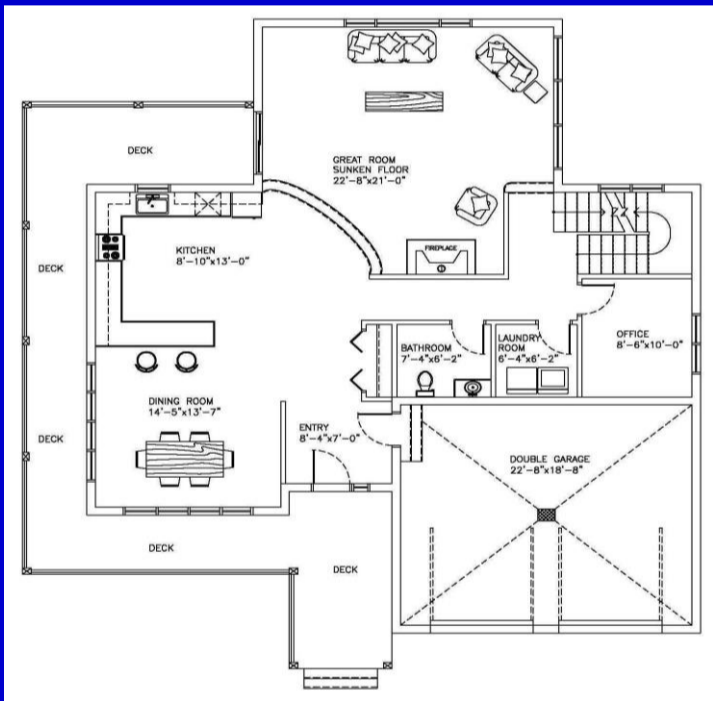
Main floor plan 1320 Sq.Ft
