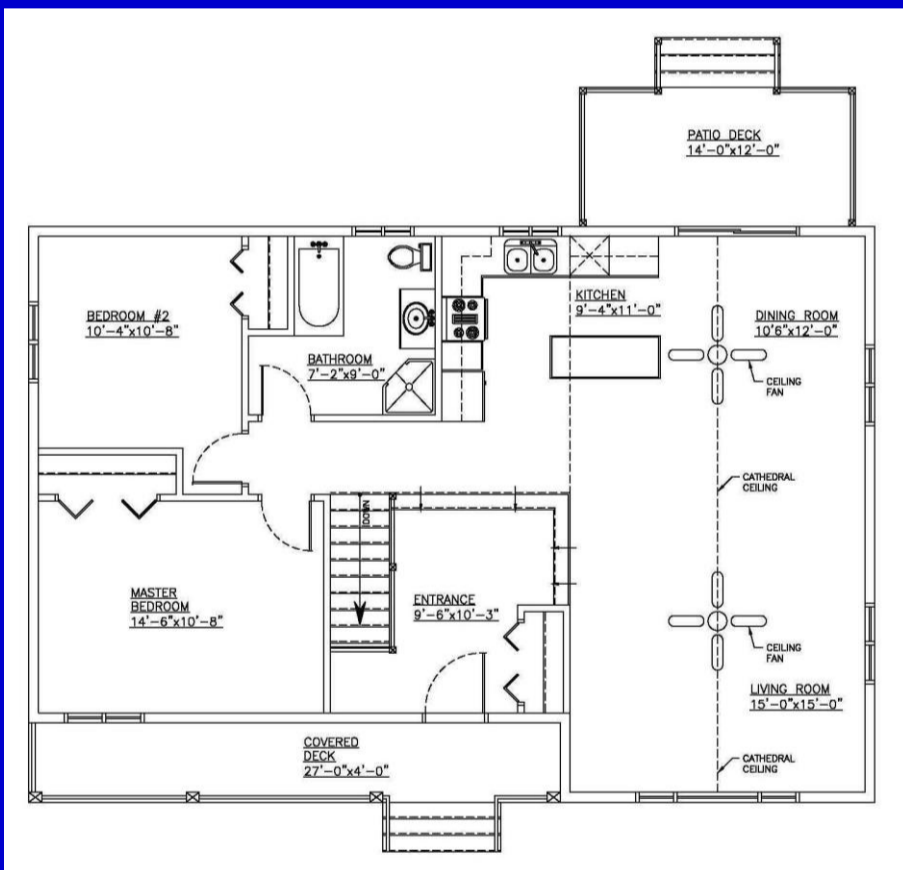
Main floor plan 1068 Sq.Ft
