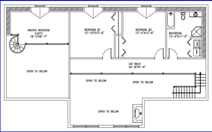
Second floor plan 955 Sq.Ft
