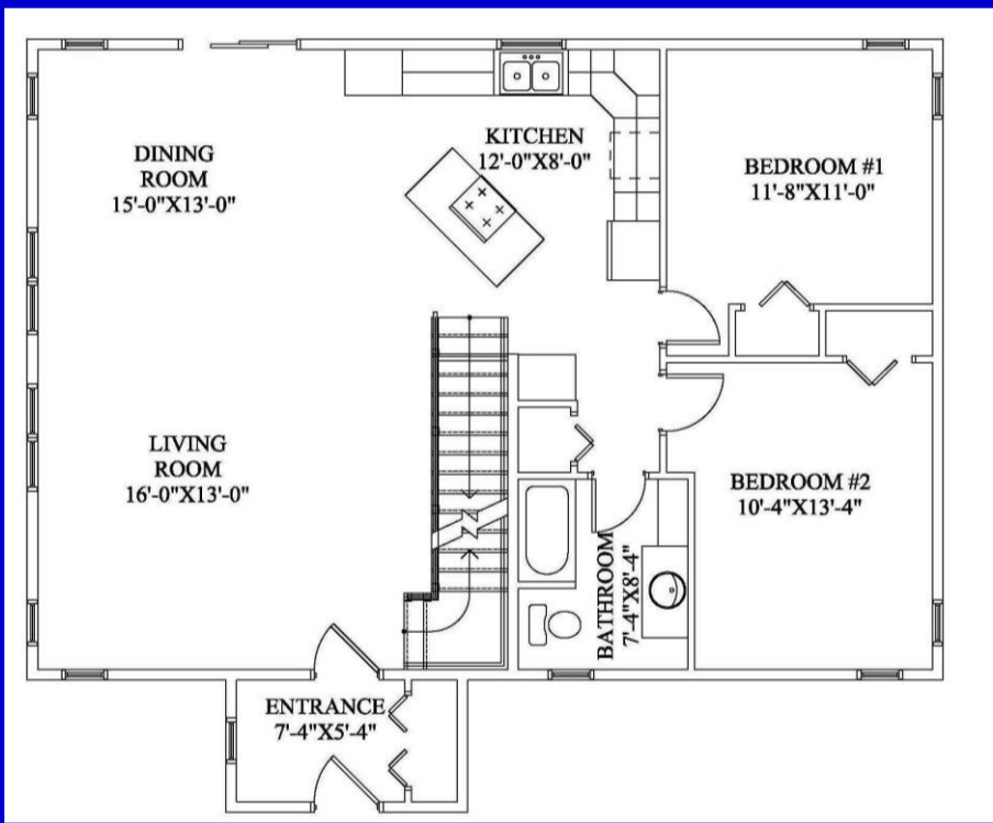
Main floor plan 1108 Sq.Ft
