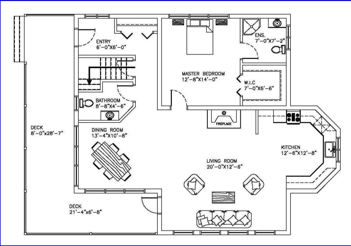
Main floor plan 1140 Sq.Ft
