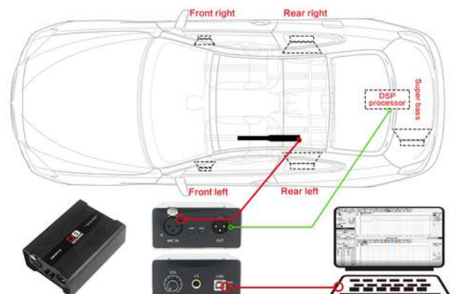
Car Audio System Measurement Connection Diagram Acoustic Measuring Instrument DBMRT2
