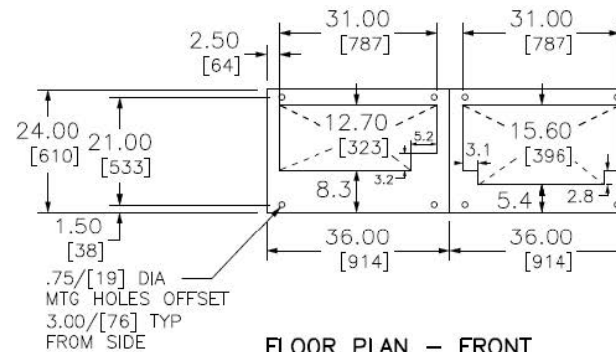
FLOOR PLAN — FRONT
