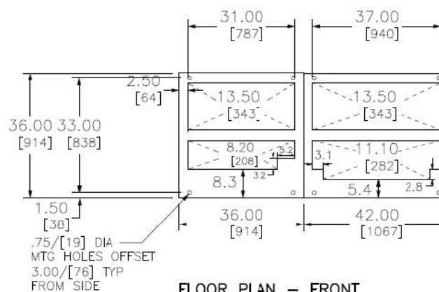
FLOOR PLAN - FRONT
