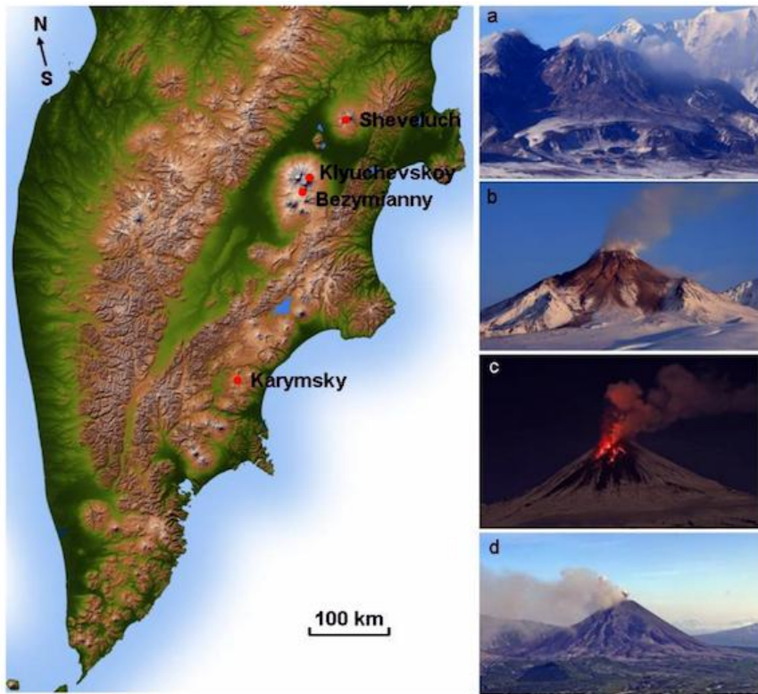
(Kamchatka and Four of its Twenty-nine Active Volcanoes)
