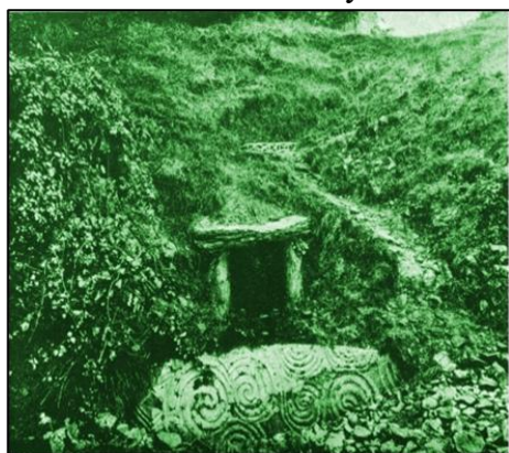
Figure 98: Unrestored entrance to New Grange. Note the cup and ring markings on the threshold.
