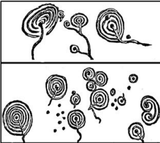
Figure 97: Cup and ring markings from Scotland (After Sir F. Simpson and Rolleston)
