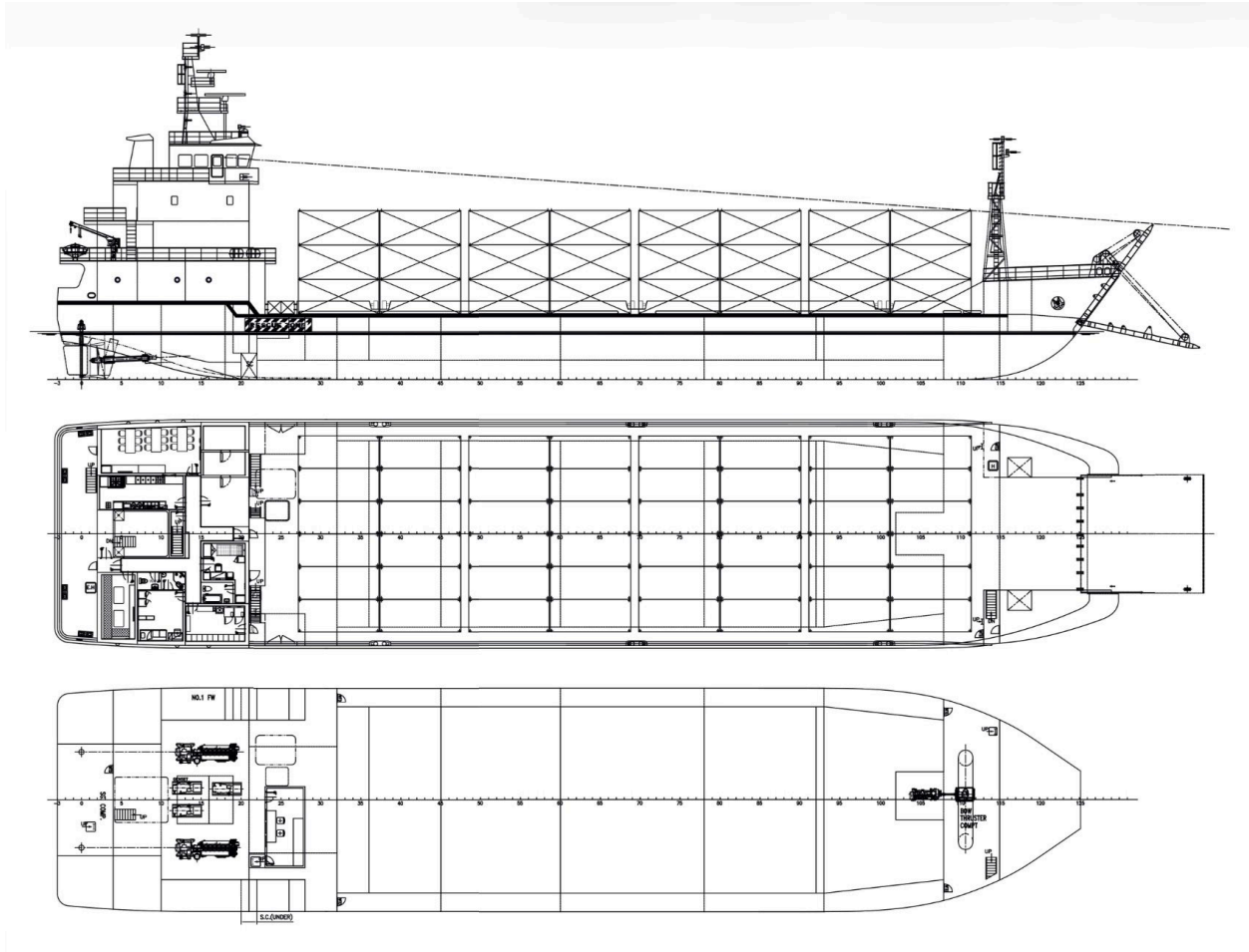
2026 BUILT 1700 DWT LANDING CRAFT
