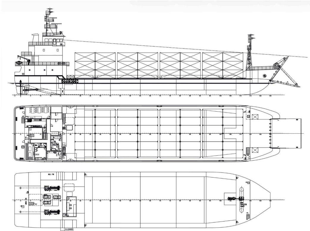
2026 NEW BUILT 80 METERS CUSTOM LANDING CRAFT
