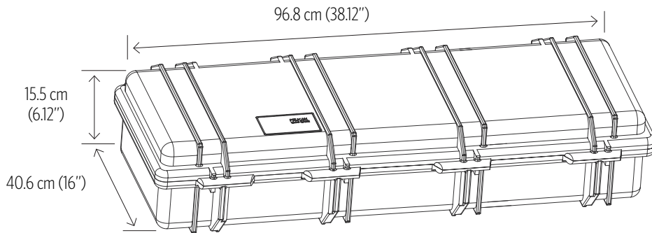
Shipping Case Pelican Model 1700 Empty Case: 7.3 kg (16.1 lbs) Shipping Weight: 18.4 kg (40.6 lbs) Shipping Dims (in cardboard box): 125 cm (49.2") x 43 cm (16.9") x 37 cm (14.6")
