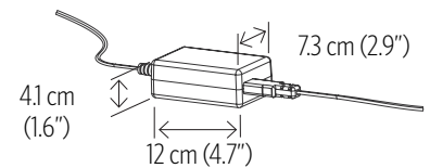
Standard 24V Power Supply 227 g (0.5 lbs)
