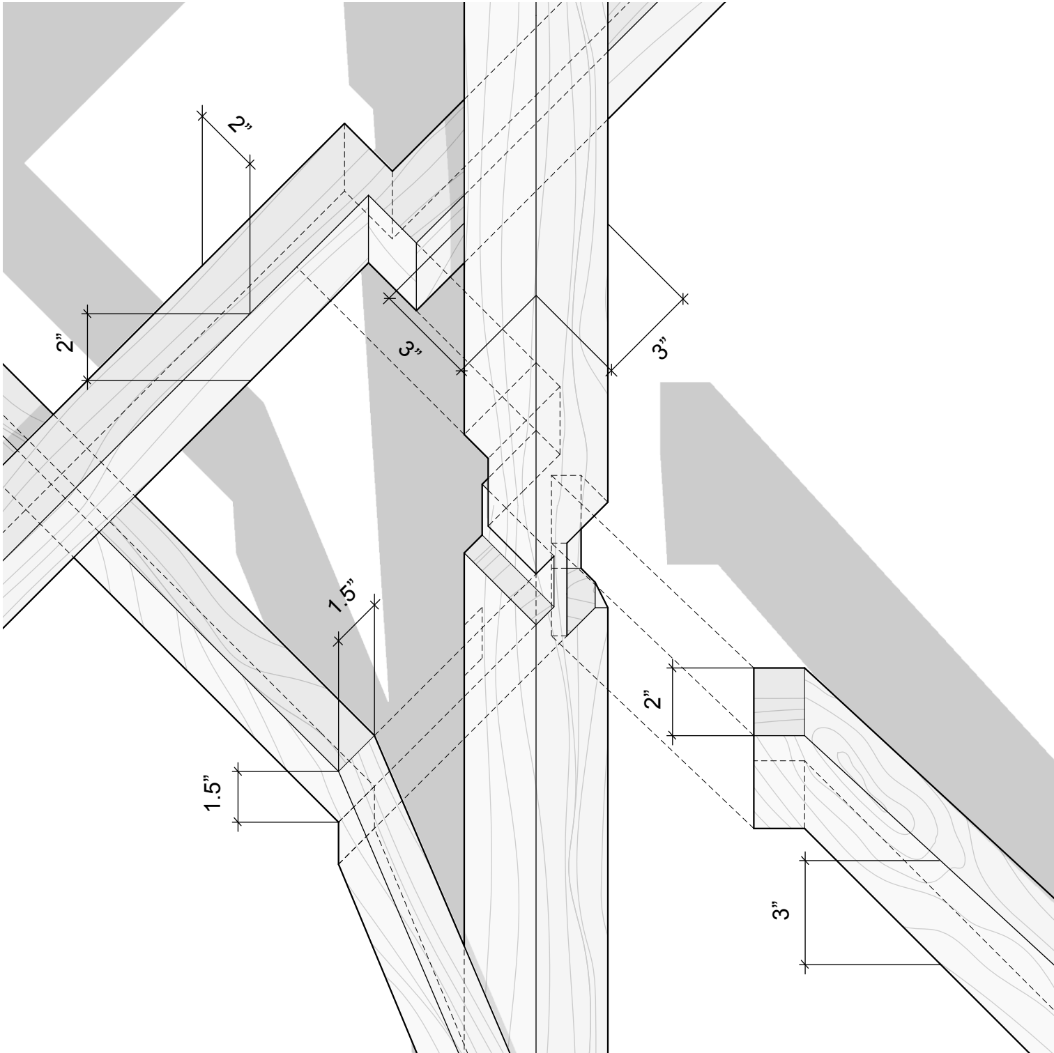
02. Redefined Vernacular Joint. Disassembled scale: 1/3'=1'=0"
