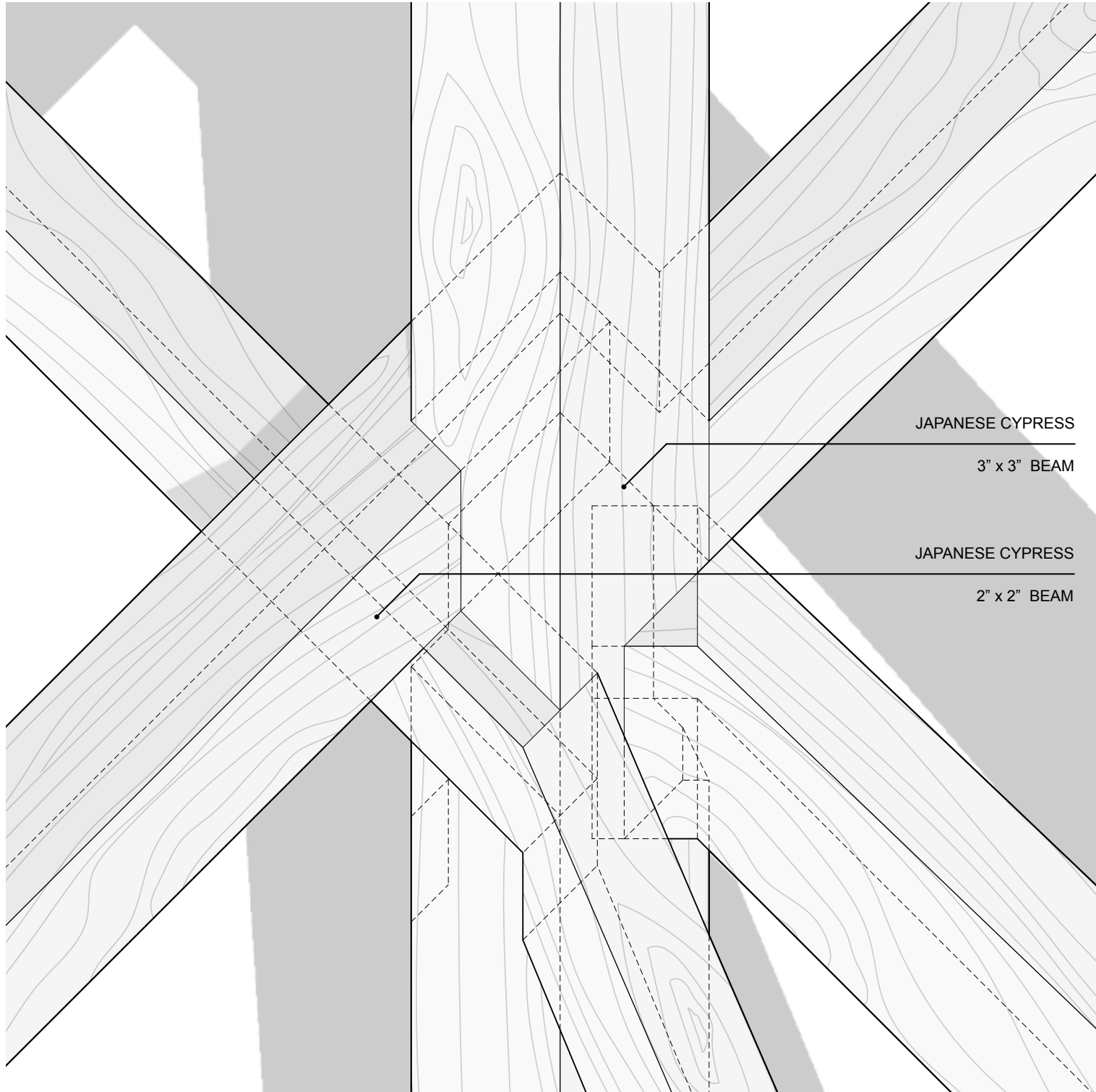
01. Redefined Vernacular Joint. Assembled scale: 1/2'=1'=0"
