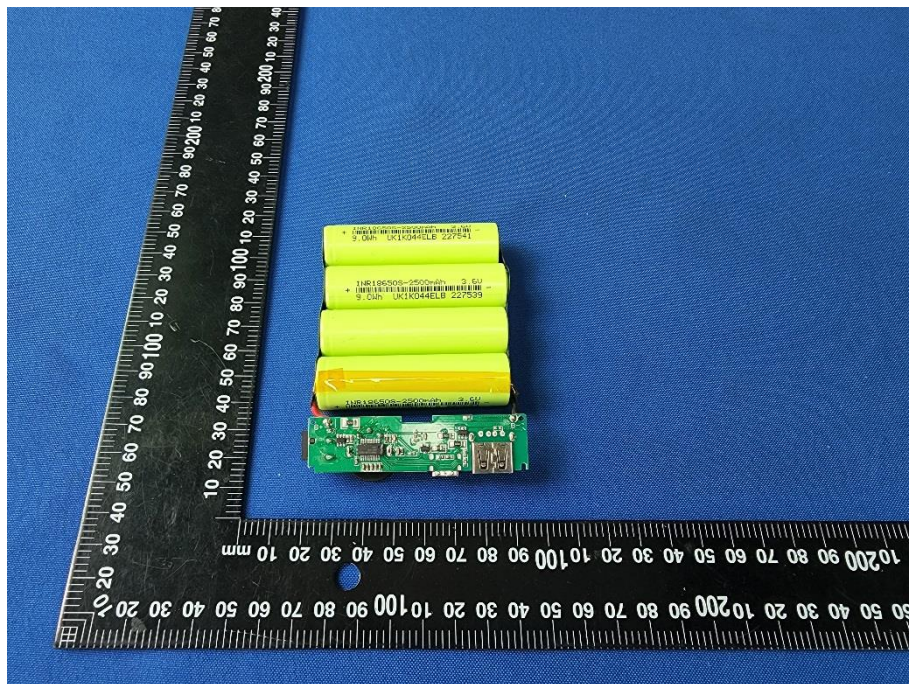
Figure 6_ Internal view for GameWarmer
