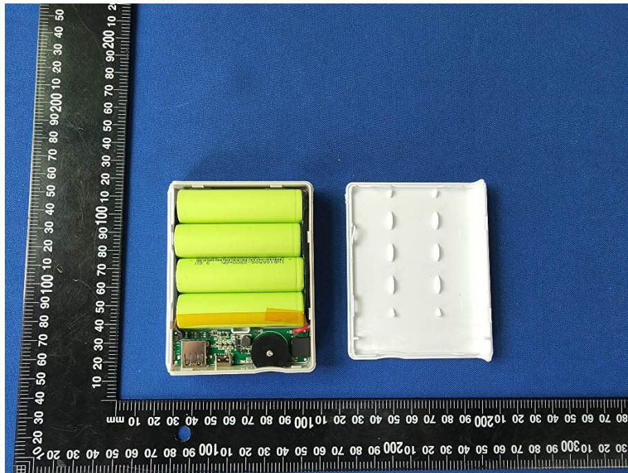
Figure 5_ Internal view for GameWarmer
