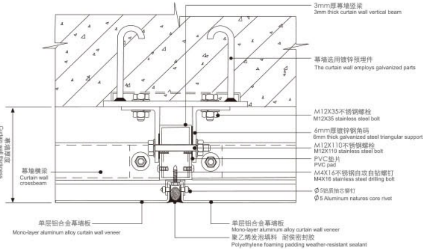
单层铝合金幕墙板安装节点图 Installation node drawing of single-layer aluminum curtain wall veneer
