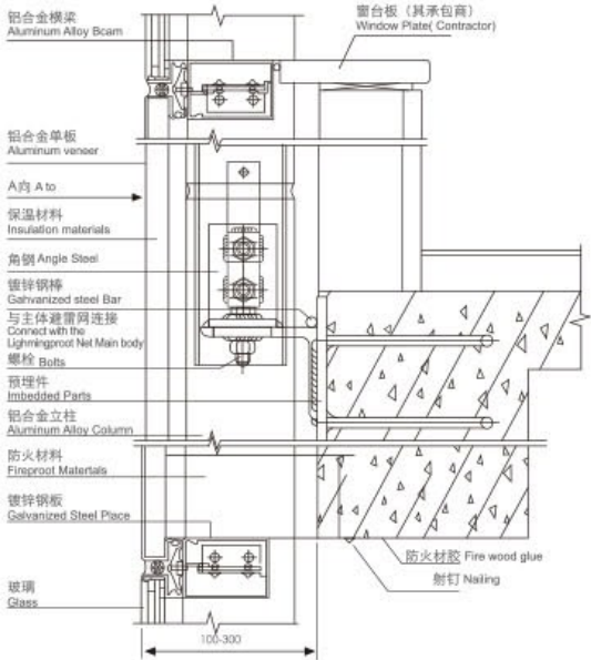
铝单板幕墙节点图 Installation node drawing of aluminum curtain wall
