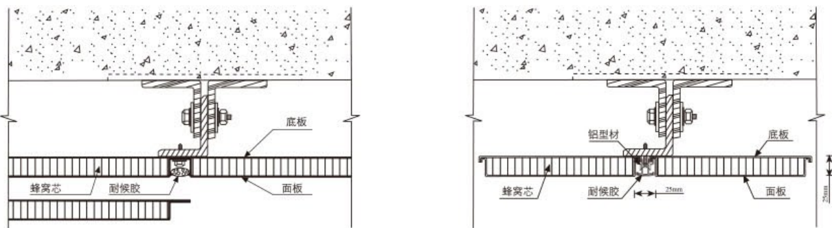
自身连接解码安装节点图 Oneself conjunction the decoding install node diagram
