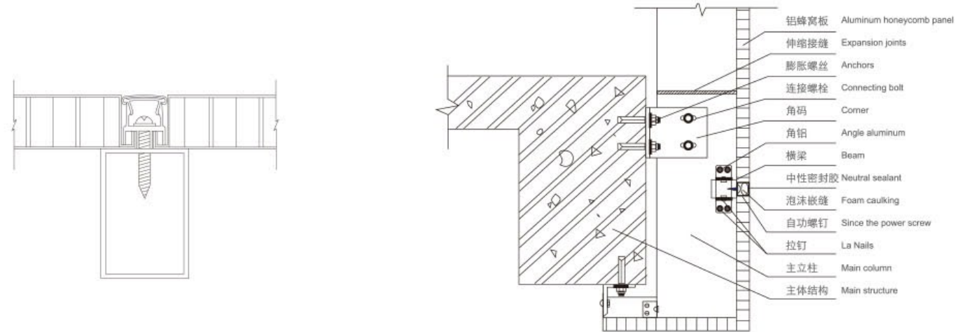
幕墙铝蜂窝板安装示意图 Curtain wall installation diagram of aluminum honeycomb panels
