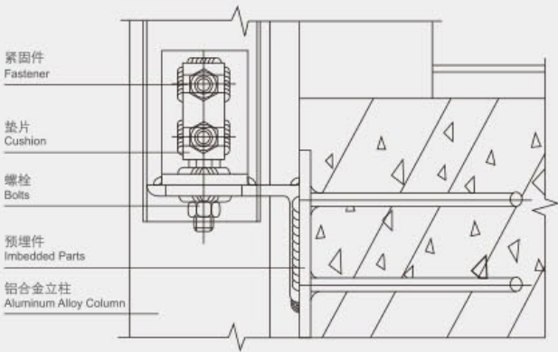
铝单板幕墙节点图 Installation node drawing of aluminum curtain wall
