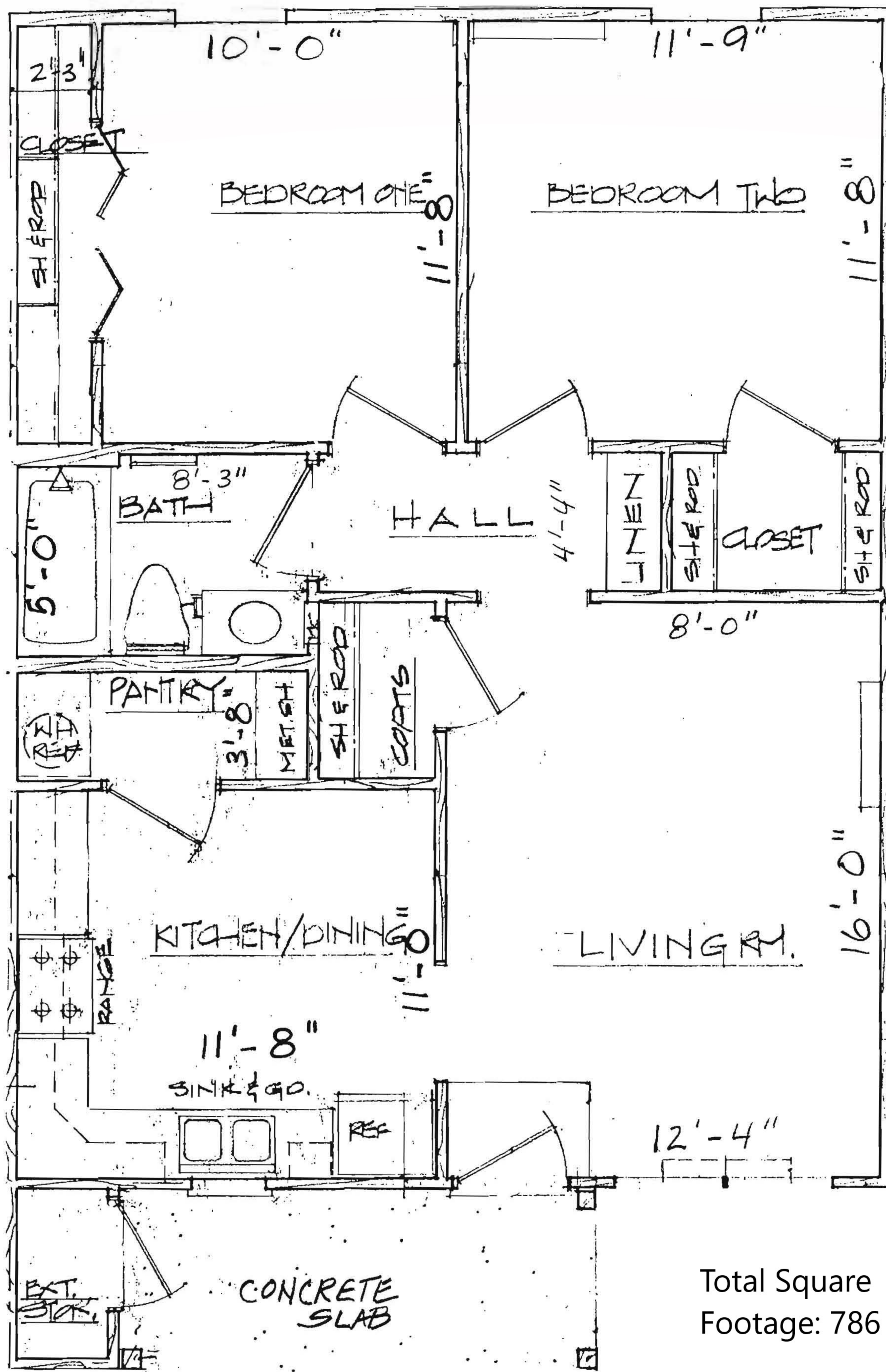
TWO BEDROOM FLOOR PLAN
