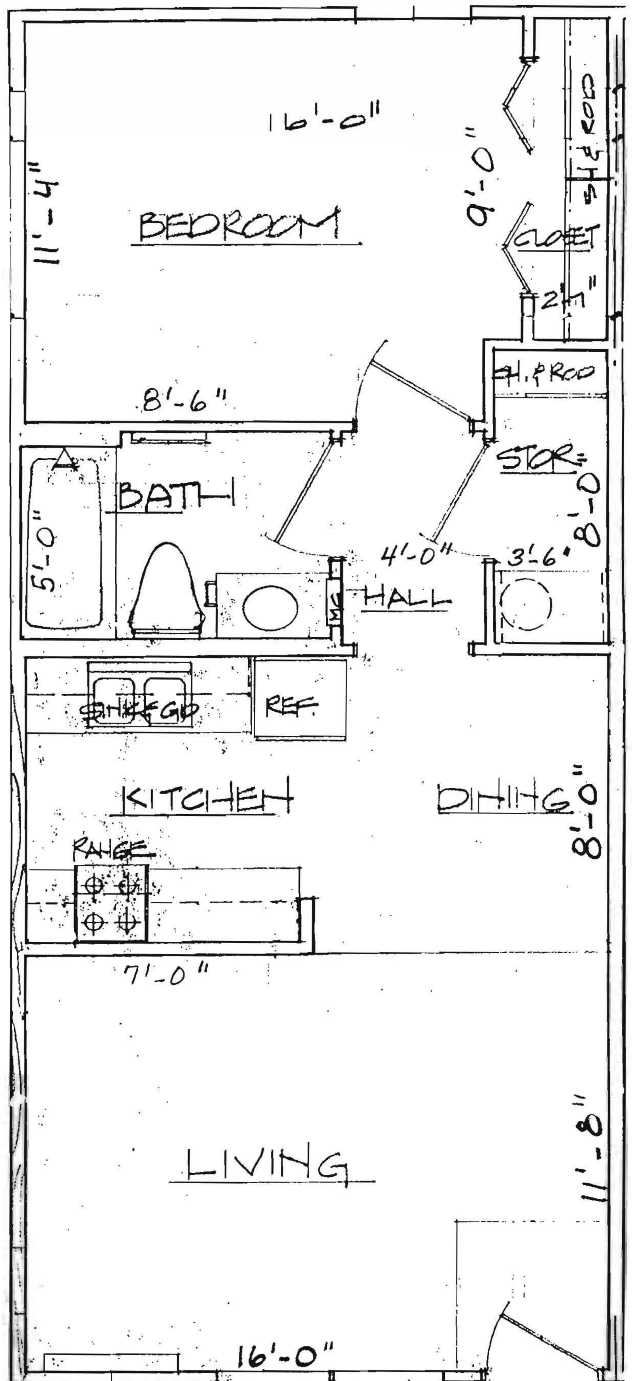
ONE BEDROOM FLOOR PLAN
