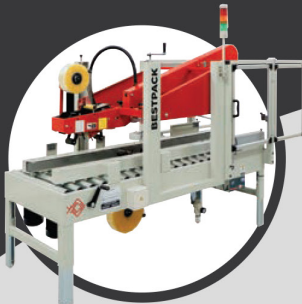
CARTON SEALING Equipment
