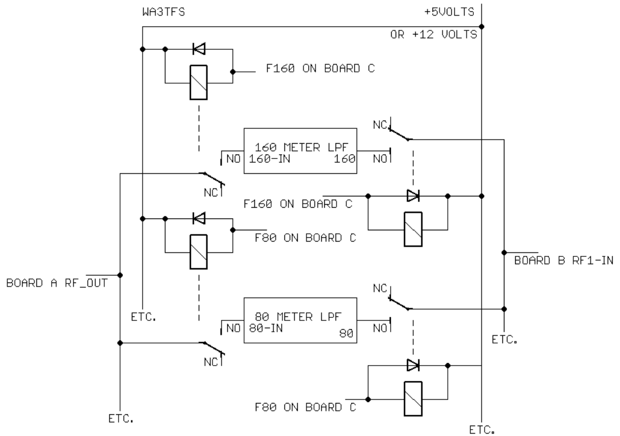
EXAMPLE OF LOW PASS FILTER RELAY SWITCHING SHOWING TWO FILTERS, JUST CONTINUE FOR OTHER FILTERS
