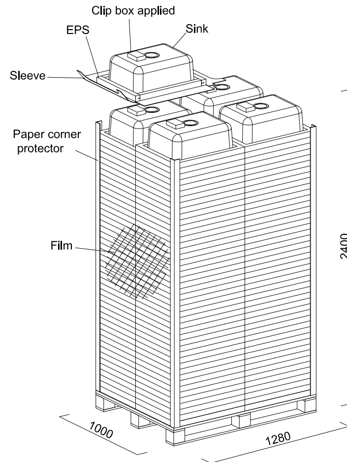
PACKAGE DIAGRAM (Waste Kit & Drain Pipe packed on separate pallet)
