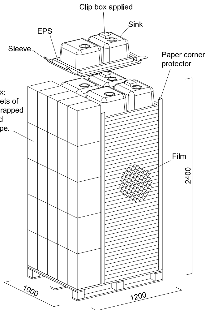
PACKAGE DIAGRAM
