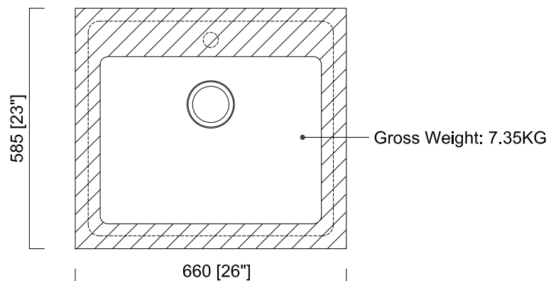
PACKAGING DIAGRAM
