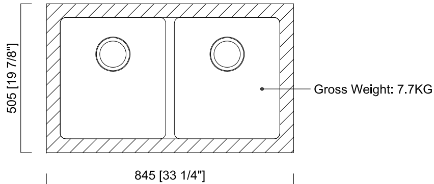
PACKAGING DIAGRAM
