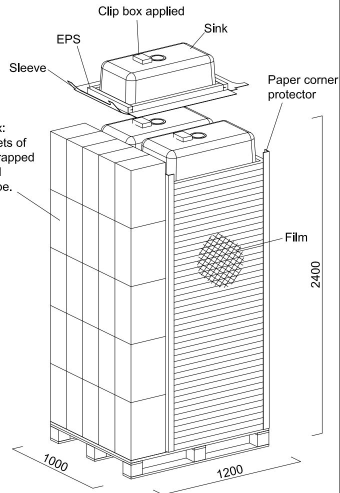
PACKAGE DIAGRAM
