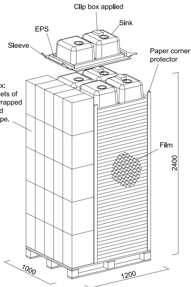
PACKAGE DIAGRAM
