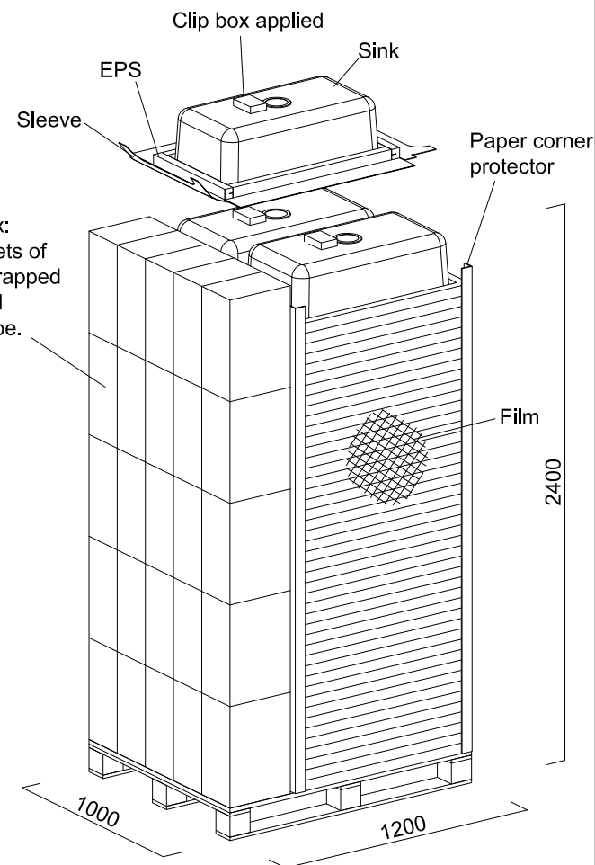
PACKAGE DIAGRAM
