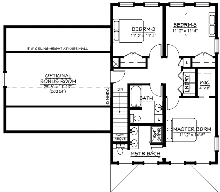
SECOND FLOOR 864 SF + OPT. 302 SF
