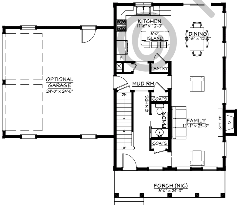
FIRST FLOOR 864 SF
