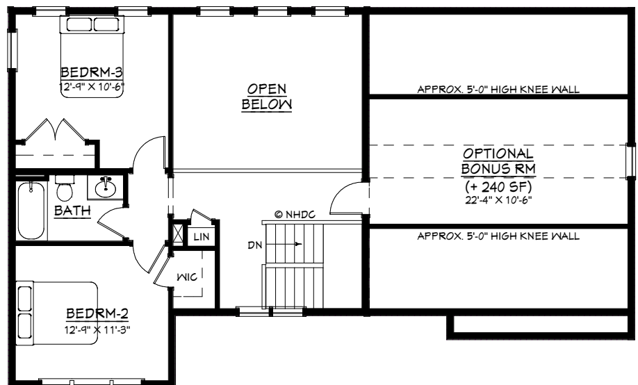
SECOND FLOOR 844 SF
