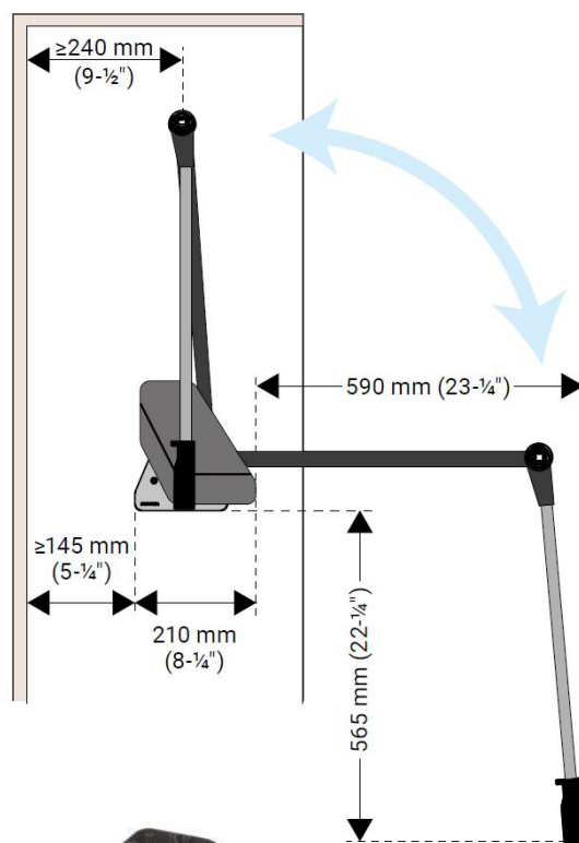
Classic Wardrobe Lift - Side View
