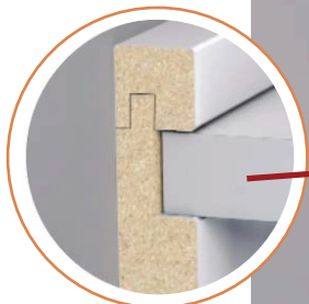
Grooved cleat system hides out of square drywall
