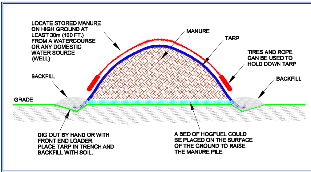
Figure 1 Field Storage of Manure
