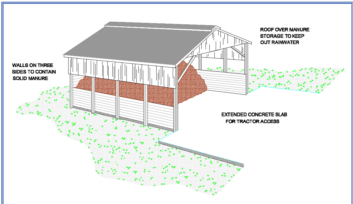
Figure 2 Example of A Solid Manure Storage Facility
