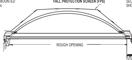
OPTIONAL ACRA-GUARD FALL PROTECTION SCREEN (FPS)
