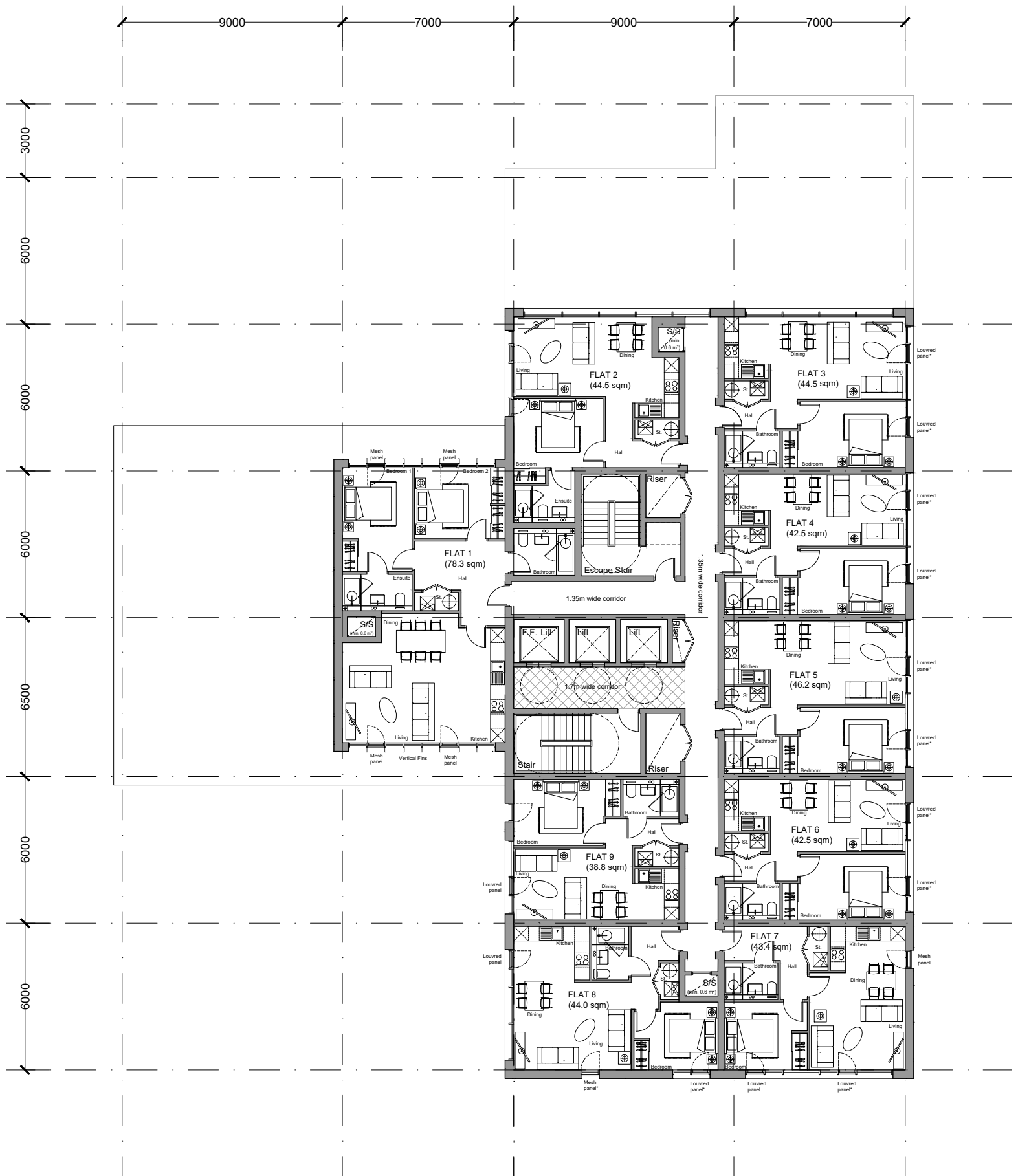
PROPOSED 23rd-27th FLOORS * - mesh and louvre panels are randomly positioned please refer to elevations for exact locations
