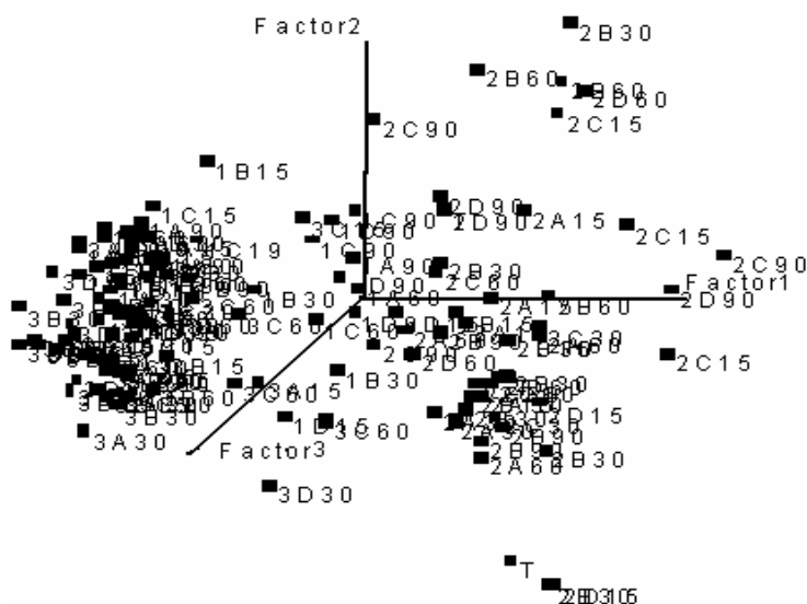
Fig 1. PCA on the data obtained from the analysis of rums by HS-MS e-nose (ions 95, 96, 109 and 110 m/z ).
