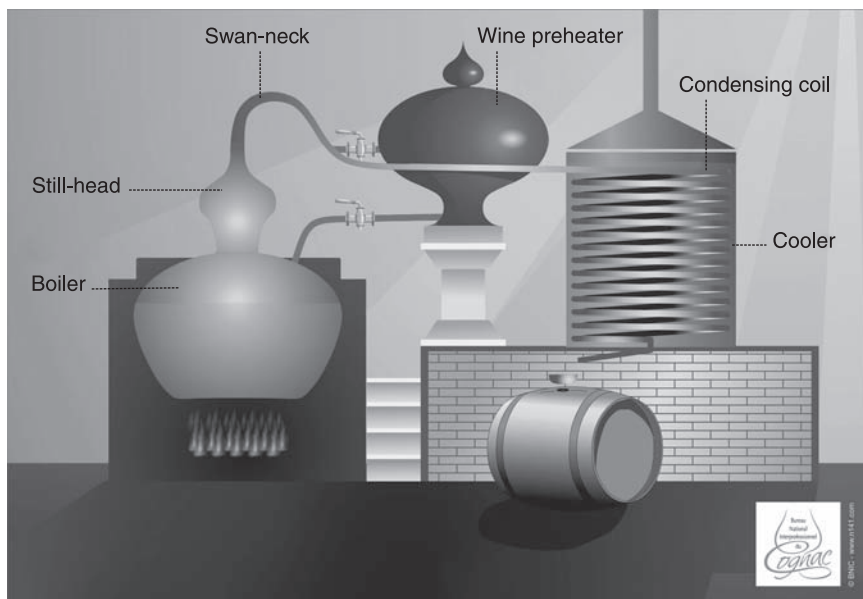
Fig. 11.3 The Charentais still: main components (© BNIC).
