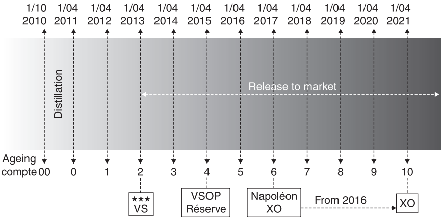
Fig. 11.4 Cognac ageing counts and designations (© BNIC).
