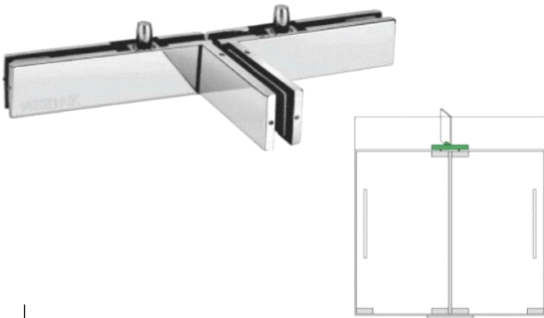
SSI 128(A) DOUBLE PANEL PATCH WITH FINIS
