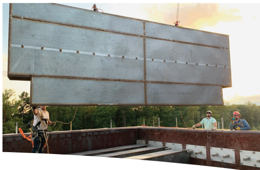
Installation of new vertical silencer panels.
