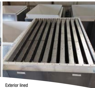
Exterior lined inlet silencer duct (FS7B)
