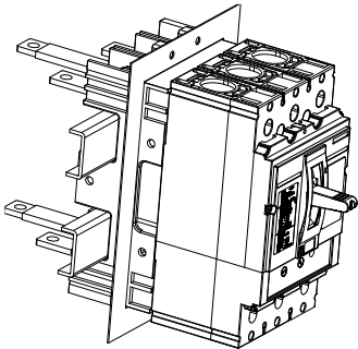
PIA22N Plug-In Base for M2 Unit: in [mm]
