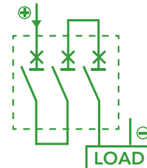
Connection D
