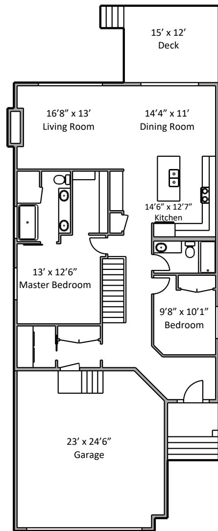
1495 sq ft main floor
