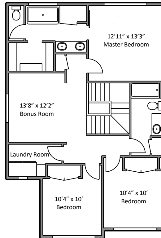
1015 sq ft upper floor
