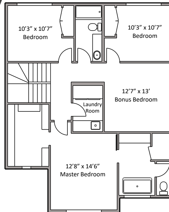
1140 sq ft upper floor
