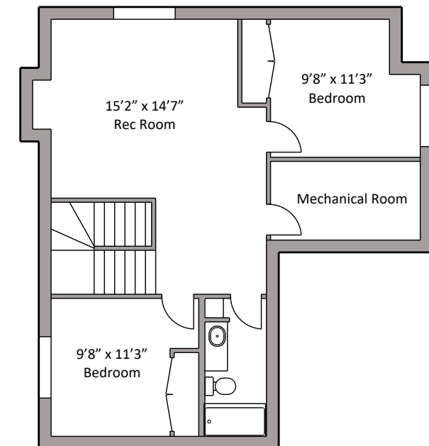
660 sq ft future basement development
