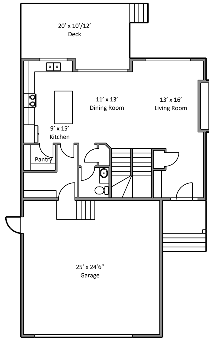
870 sq ft main floor
